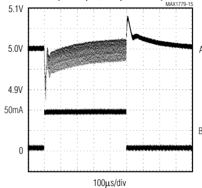
LOAD TRANSIENT (L = 10μH, 500μs PULSE)
