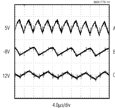
RIPPLE WAVEFORMS
